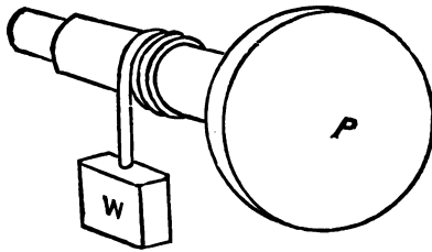
FIG. 202.—Diagram Illustrating the Theory of Torque.
